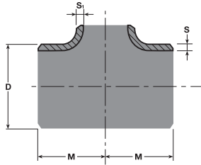
Weights of Reducing Tees: see Equal Tees
